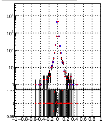
Legend: DQM_TT_mkFit-DQM_lowptq_orig (Black line) DQM_TT_mkFit-DQM_lowptq_modi3 (Red line)
