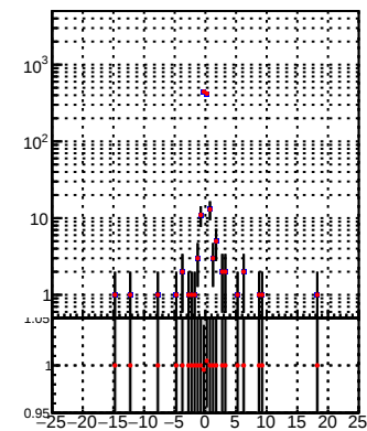
Legend: DQM_TT_mkFit-DQM_lowptq_orig (black histogram) DQM_TT_mkFit-DQM_lowptq_modi3 (red line)
