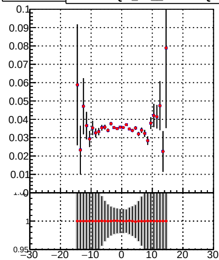
—•— DQM_TT_mkFit-DQM_lowptq_orig —•— DQM_TT_mkFit-DQM_lowptq_modi3
