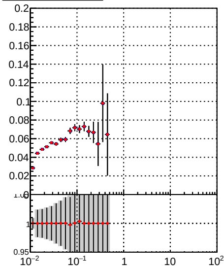
—•— DQM_TT_mkFit-DQM_lowptq_orig —•— DQM_TT_mkFit-DQM_lowptq_modi3
