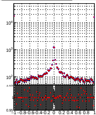
— DQM_TT_mkFit-DQM_lowptq_orig — DQM_TT_mkFit-DQM_lowptq_modi3
