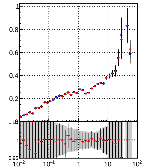
—•— DQM_TT_mkFit-DQM_lowptq_orig —•— DQM_TT_mkFit-DQM_lowptq_modi3
