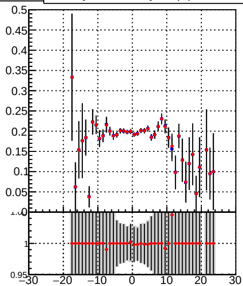
Efficiency vs vertpos — DQM_TT_mkFit-DQM_lowptq_orig — DQM_TT_mkFit-DQM_lowptq_modi3
