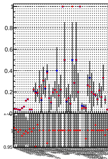
Fake rate vs. —●— DQM TT mkFit-DQM_lowptq_orig —●— DQM TT mkFit-DQM_lowptq_modi3
