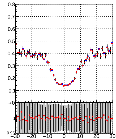
—●— DQM_TT_mkFit-DQM_lowptq_orig —●— DQM_TT_mkFit-DQM_lowptq_modi3
