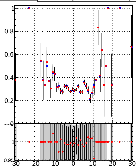
—•— DQM_TT_mkFit-DQM_lowptq_orig —•— DQM_TT_mkFit-DQM_lowptq_modi3
