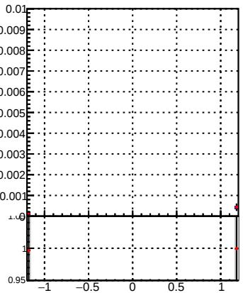
Duplicates Rate vs Dz(PV)
