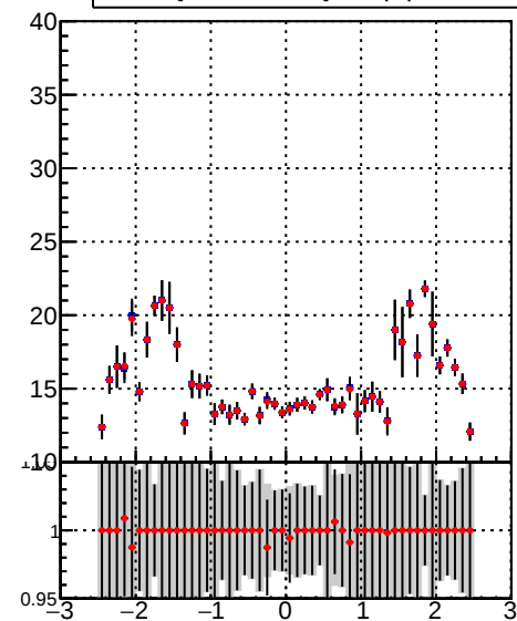
— DQM_TT_mkFit-DQM_lowptq_orig — DQM_TT_mkFit-DQM_lowptq_modi3
