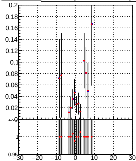
Fake rate vs v Legend: DQM_TT_mkFit-DQM_lowptq_orig DQM_TT_mkFit-DQM_lowptq_modi3
