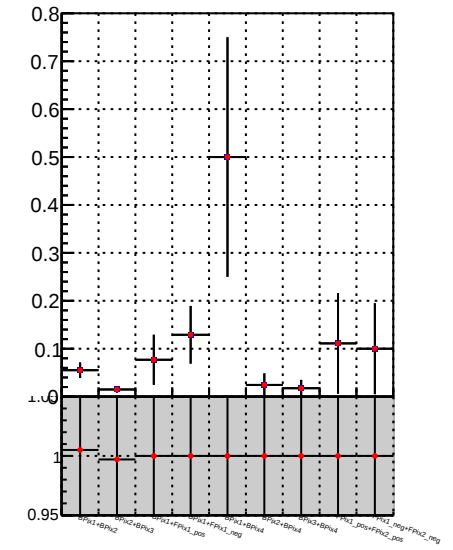
Fake rate vs. — DQM_TT_mkFit-DQM_lowptq_orig — DQM_TT_mkFit-DQM_lowptq_modi3
