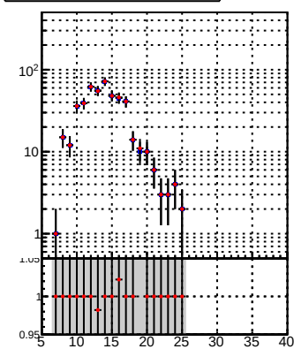
Legend: DQM_TT_mkFit-DQM_lowptq_orig (blue line with dots), DQM_TT_mkFit-DQM_lowptq_modi3 (red line with dots)
