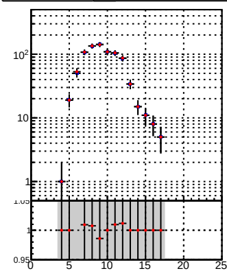
Legend: DQM_TT_mkFit-DQM_lowptq_orig (blue line with dots), DQM_TT_mkFit-DQM_lowptq_modi3 (red line with dots)
