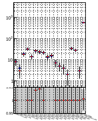
N of reco track vs. \chi^2 — mkFit-DQM_lowptq_orig — mkFit-DQM_lowptq_mod3
