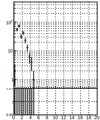
N of reco track vs. \chi^2 — DQM TT mkFit-DQM_lowptq_orig — DQM TT mkFit-DQM_lowptq_modi3
