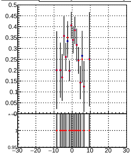
Fake rate vs vertpos DQM_TT_mkFit-DQM_lowptq_orig DQM_TT_mkFit-DQM_lowptq_modi3
