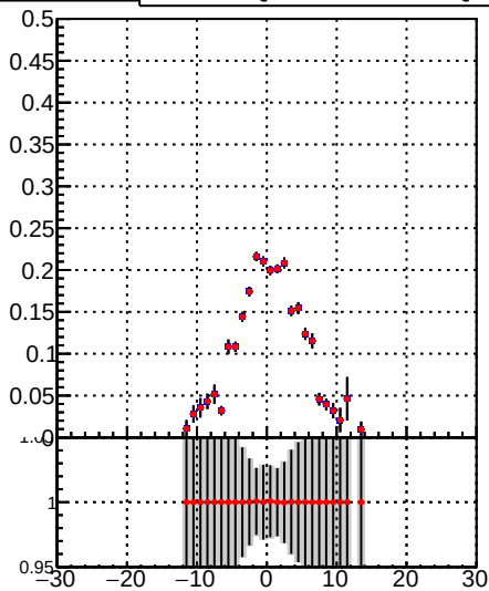
Fake rate vs v — DQM_TT_mkFit-DQM_lowptq_orig — DQM_TT_mkFit-DQM_lowptq_modi3
