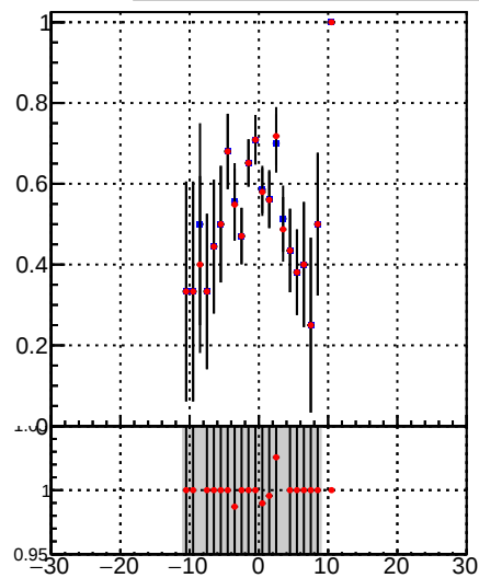
—■— DQM_TT_mkFit-DQM_lowptq_orig —■— DQM_TT_mkFit-DQM_lowptq_modi3
