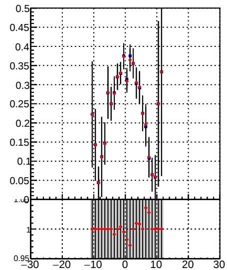
Fake rate vs d —●— DQM TT mkFit-DQM_lowptq_orig —●— DQM TT mkFit-DQM_lowptq_modi3
