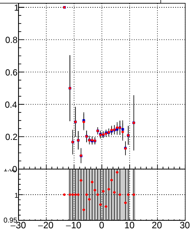
Legend: ■ DQM_TT_mkFit-DQM_lowptq_orig ● DQM_TT_mkFit-DQM_lowptq_modi3
