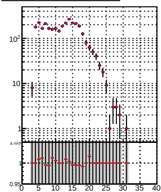
N of reco track vs hit DQM_TT_mkFit-DQM_lowptq_orig DQM_TT_mkFit-DQM_lowptq_modi3
