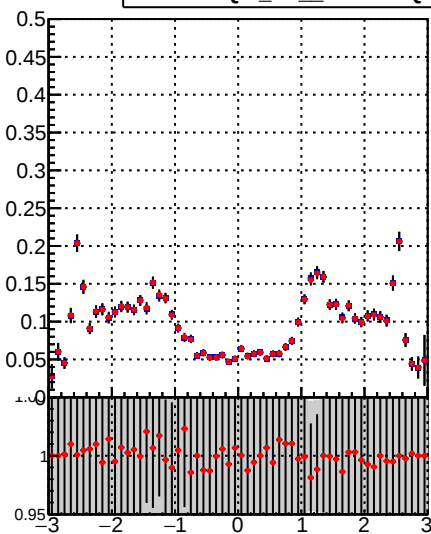
—■— DQM_TT_mkFit-DQM_lowptq_orig —●— DQM_TT_mkFit-DQM_lowptq_modi3
