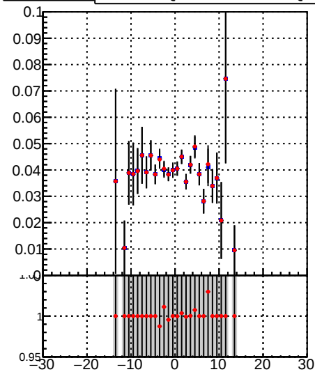
Legend: —•— DQM_TT_mkFit-DQM_lowptq_orig —•— DQM_TT_mkFit-DQM_lowptq_modi3 Fake rate vs v
