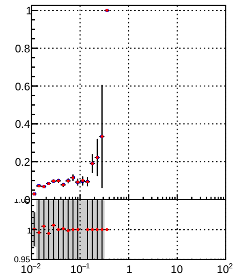
Legend: —•— DQM_TT_mkFit-DQM_lowptq_orig —•— DQM_TT_mkFit-DQM_lowptq_modi3 Fake rate vs v
