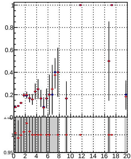
Fake rate vs. —●— DQM_TT_mkFit-DQM_lowptq_orig —●— DQM_TT_mkFit-DQM_lowptq_mod3
