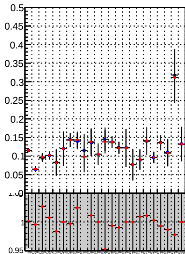
Fake rate vs. —●— DQM_TT_mkFit-DQM_lowptq_orig —●— DQM_TT_mkFit-DQM_lowptq_mod3
