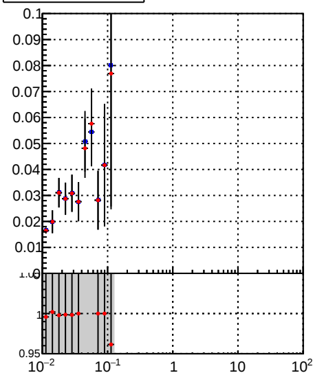
—•— DQM_TT_mkFit-DQM_lowptq_orig —•— DQM_TT_mkFit-DQM_lowptq_modi3
