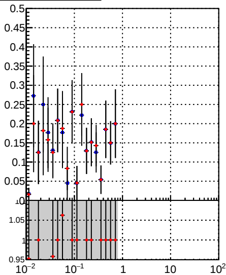
— DQM_TT_mkFit-DQM_lowptq_orig — DQM_TT_mkFit-DQM_lowptq_modi3
