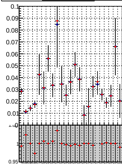
Fake rate vs. —•— DQM TT mkFit-DQM_lowptq_orig —•— DQM TT mkFit-DQM_lowptq_modi3
