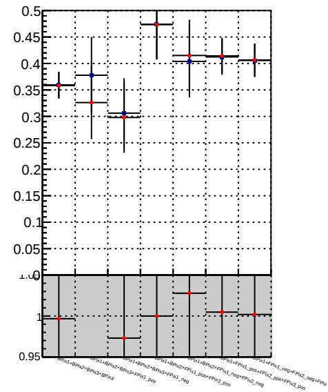
Fake rate vs. —●— DQM TT mkFit-DQM_lowptq_orig —●— DQM TT mkFit-DQM_lowptq_modi3
