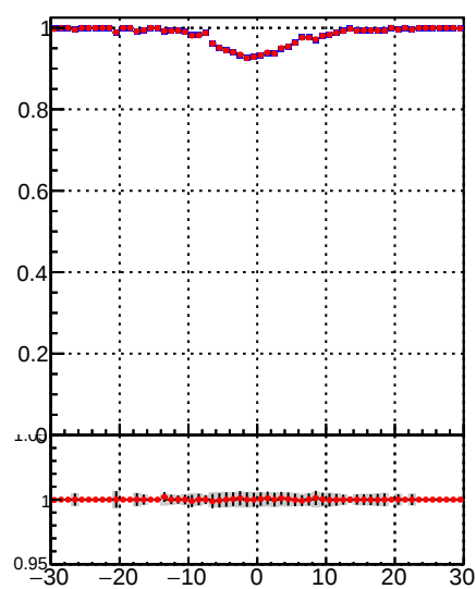
—•— DQM_TT_mkFit-DQM_lowptq_orig —•— DQM_TT_mkFit-DQM_lowptq_modi3
