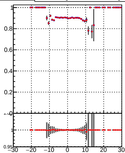
—■— DQM_TT_mkFit-DQM_lowptq_orig —●— DQM_TT_mkFit-DQM_lowptq_mod3
