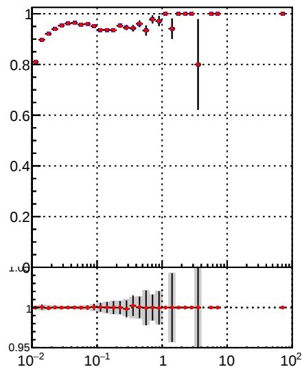
—■— DQM_TT_mkFit-DQM_lowptq_orig —●— DQM_TT_mkFit-DQM_lowptq_mod3
