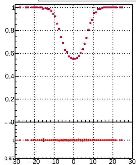
█ DQM_TT_mkFit-DQM_lowptq_orig █ DQM_TT_mkFit-DQM_lowptq_modi3
