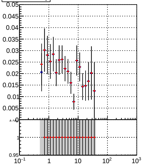
DQM_TT_mkFit-DQM_lowptq_orig DQM_TT_mkFit-DQM_lowptq_modi3
