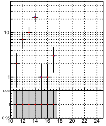
■ DQM_TT_mkFit-DQM_lowptq_orig ■ DQM_TT_mkFit-DQM_lowptq_modi3
