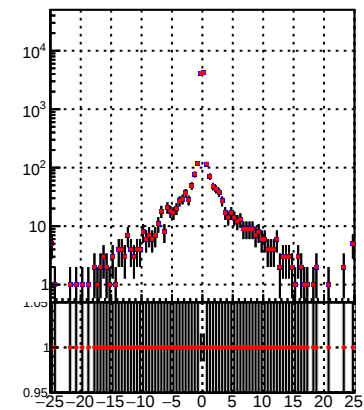
N of sim Legend: DQM_TT_mkFit-DQM_lowptq_orig DQM_TT_mkFit-DQM_lowptq_modi3
