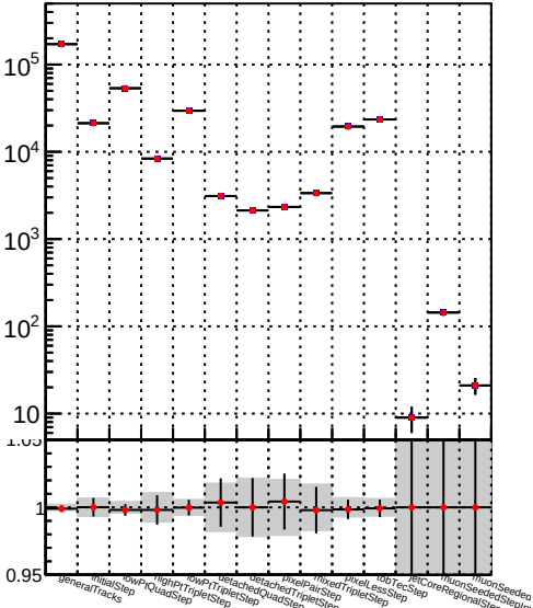
Number —●— DQM_TT__mkFit-DQM_lowptq_modi3
