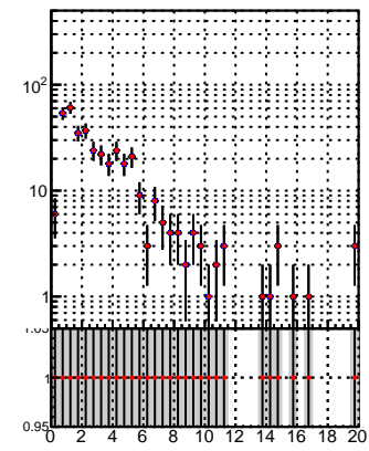
N of reco track vs. \chi^2 for DQM TT mkFit-DQM_lowptq_orig and DQM TT mkFit-DQM_lowptq_mod3
