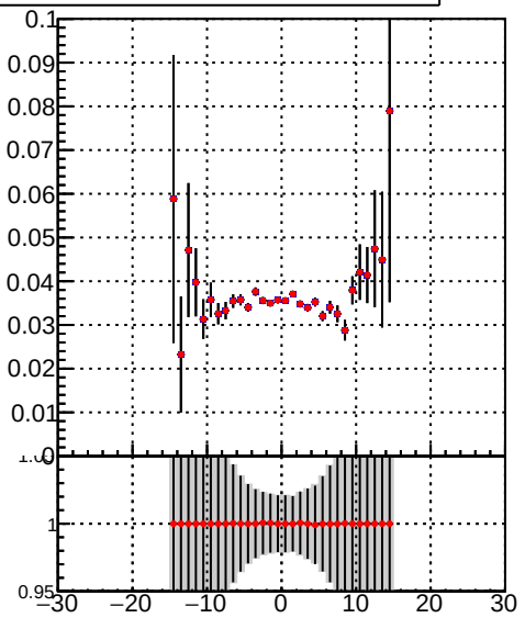
Efficiency vs. sim PV z Legend: DQM_TT_mkFit-DQM_lowptq_orig (grey shaded region) DQM_TT_mkFit-DQM_lowptq_modi3 (red crosses)
