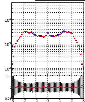
N of reco track vs \eta Legend: DQM_TT_mkFit-DQM_lowptq_orig (blue line) DQM_TT_mkFit-DQM_lowptq_modi3 (red line)
