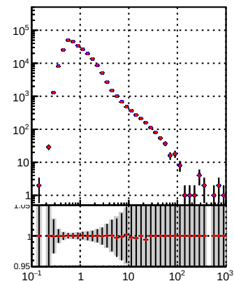
DQM_TT_mkFit-DQM_lowptq_orig DQM_TT_mkFit-DQM_lowptq_modi3
