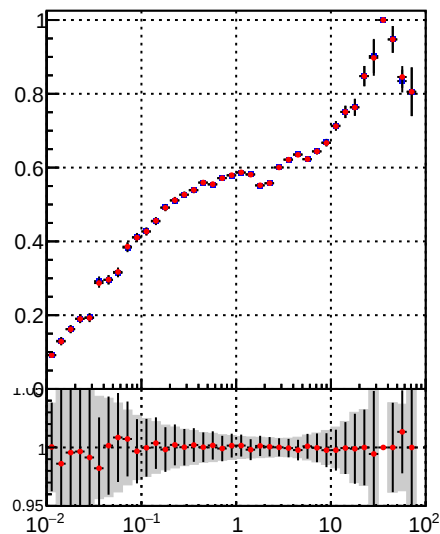
—•— DQM_TT_mkFit-DQM_lowptq_orig —•— DQM_TT_mkFit-DQM_lowptq_modi3
