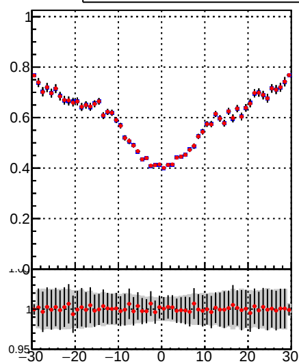
—•— DQM_TT_mkFit-DQM_lowptq_orig —•— DQM_TT_mkFit-DQM_lowptq_modi3
