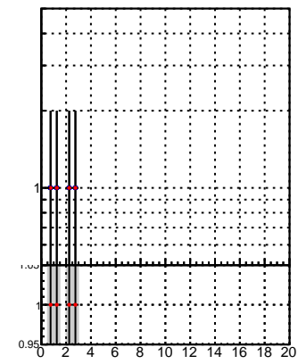
N of reco track vs. \chi^2 for DQM TT and mkFit-DQM_lowptq_modi3
