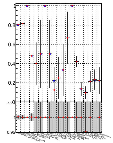
Fake rate vs. — \bullet DQM TT mkFit-DQM_lowptq_orig — \bullet DQM TT mkFit-DQM_lowptq_modi3
