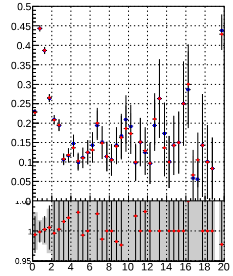
Fake rate vs. — \bullet DQM TT mkFit-DQM_lowptq_orig — \bullet DQM TT mkFit-DQM_lowptq_modi3
