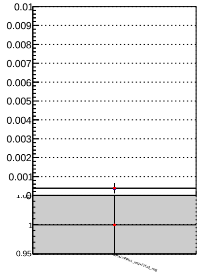
Fake rate vs. — \bullet DQM TT mkFit-DQM_lowptq_orig — \bullet DQM TT mkFit-DQM_lowptq_modi3
