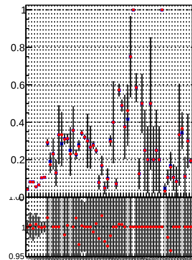
Fake rate vs. —●— DQM TT mkFit-DQM_lowptq_orig —●— DQM TT mkFit-DQM_lowptq_mod3
