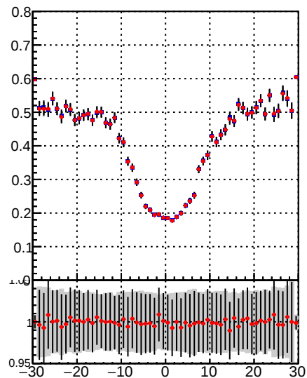
—●— DQM_TT_mkFit-DQM_lowptq_orig —●— DQM_TT_mkFit-DQM_lowptq_modi3
