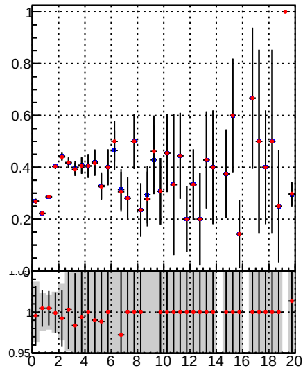
Fake rate vs. —●— DQM TT mkFit-DQM_lowptq_orig —●— DQM TT mkFit-DQM_lowptq_mod3
