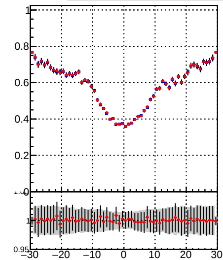
—•— DQM_TT_mkFit-DQM_lowptq_orig —•— DQM_TT_mkFit-DQM_lowptq_modi3
