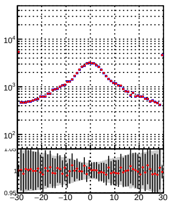
N of associated (recoToSlim) looped tracks vs transverse ref point position
