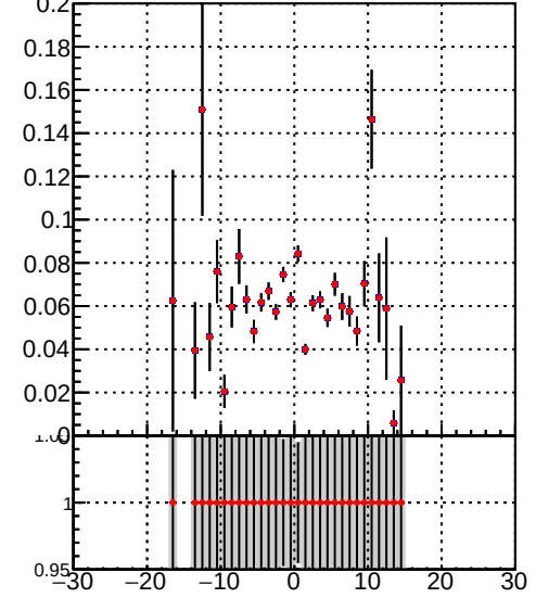
Efficiency vs. sim PV z — DQM_TT_mkFit-DQM_lowptq_orig — DQM_TT_mkFit-DQM_lowptq_modi3
