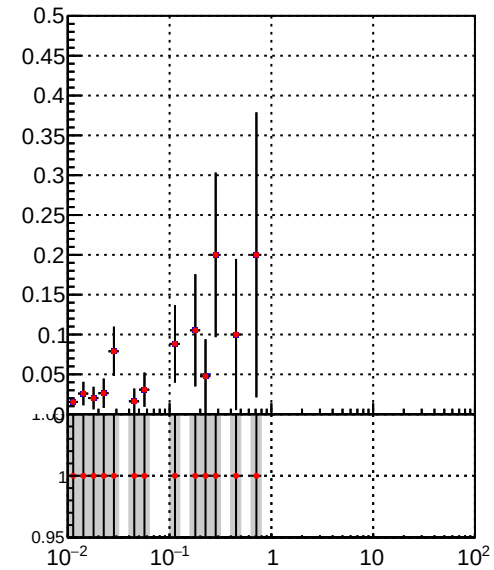
Efficiency vs. sim PV z — DQM_TT_mkFit-DQM_lowptq_orig — DQM_TT_mkFit-DQM_lowptq_modi3
