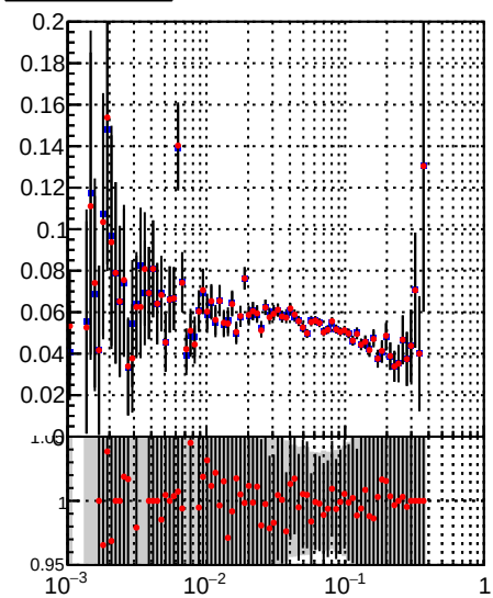
—■— DQM_TT_mkFit-DQM_lowptq_orig —●— DQM_TT_mkFit-DQM_lowptq_modi3
